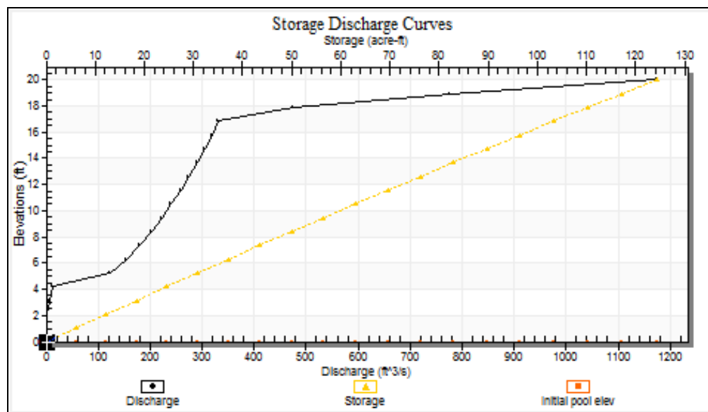
Figure 10 Reservoir Storage-Elevation-Discharge
