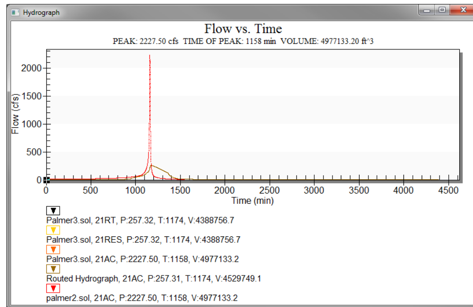
Figure 11 Both hydrographs at outlet 21AC
